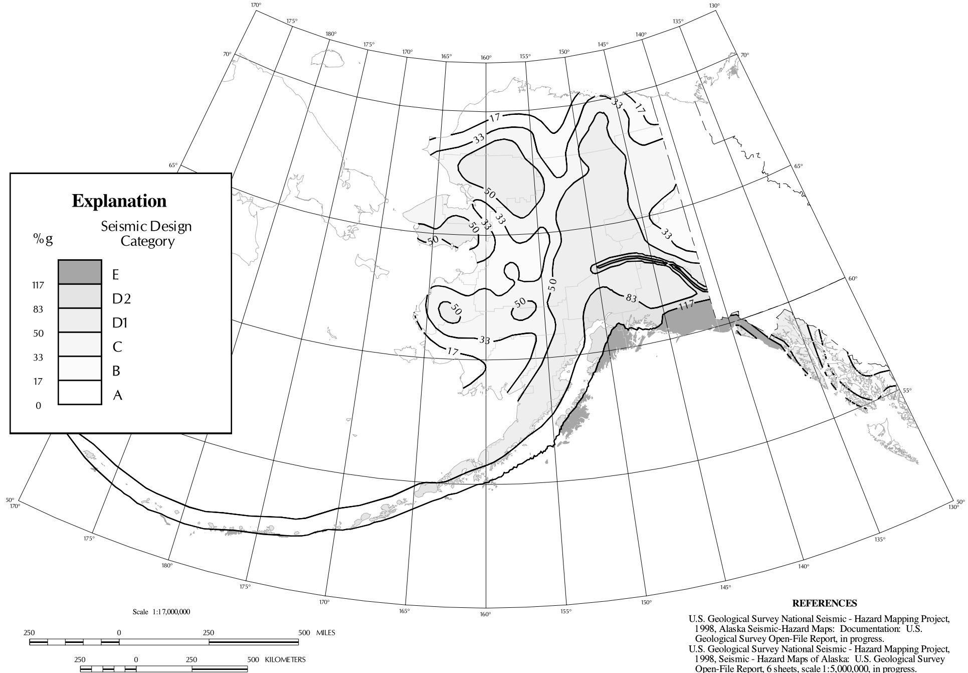
FIGURE R301.2B INTERNATIONAL RESIDENTIAL CODE SEISMIC DESIGN CATEGORIES - SITE CLASS D
